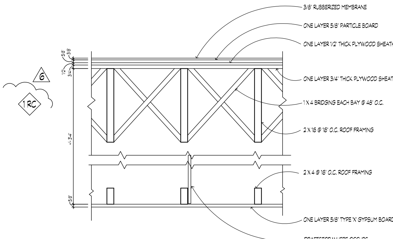
ROOF / CEILING (EXISTING COND.)
