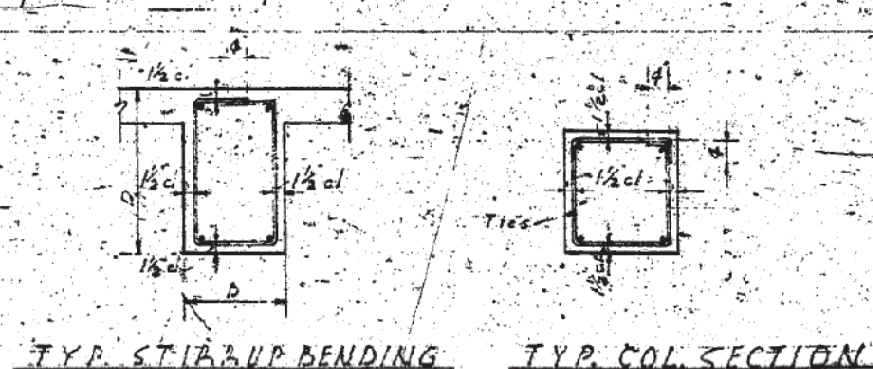
(E) CONC. BEAM AND COLUMN, TYP. (TAKEN FROM ORIG. DRAWINGS)
